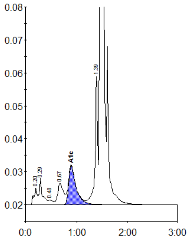
Peak table - ID: 10122360
