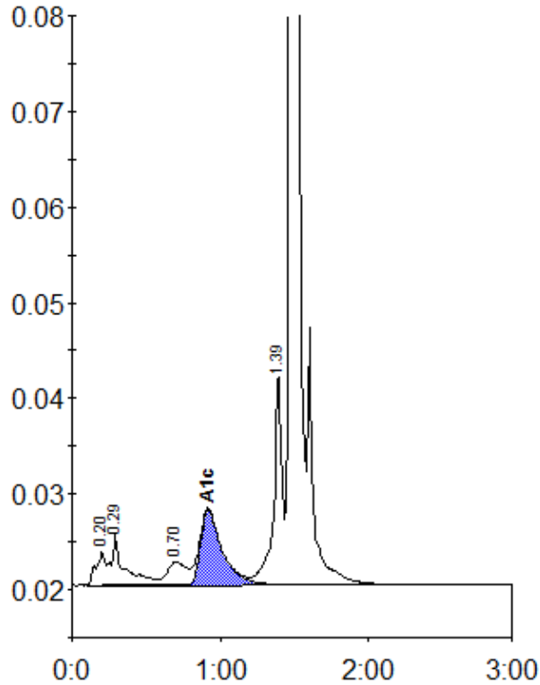
Peak table - ID: 10122714
