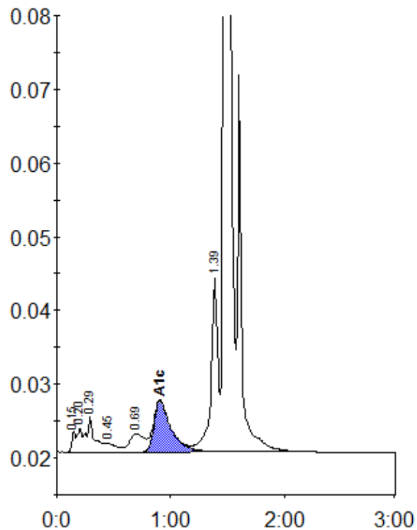
Peak table - ID: 10124710
