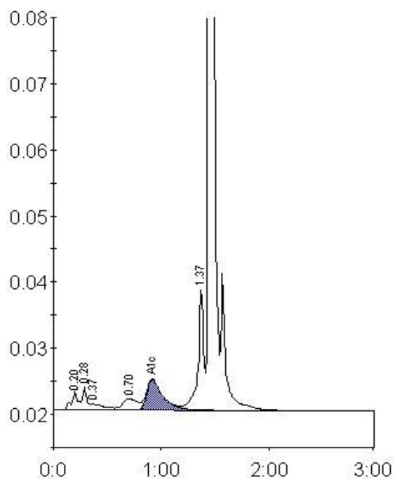
Peak table - ID: 10128816
