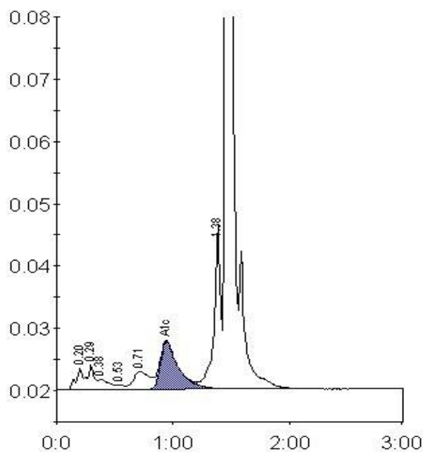
Peak table - ID: 10128934
