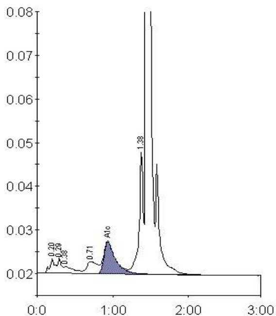
Peak table - ID: 10128975
