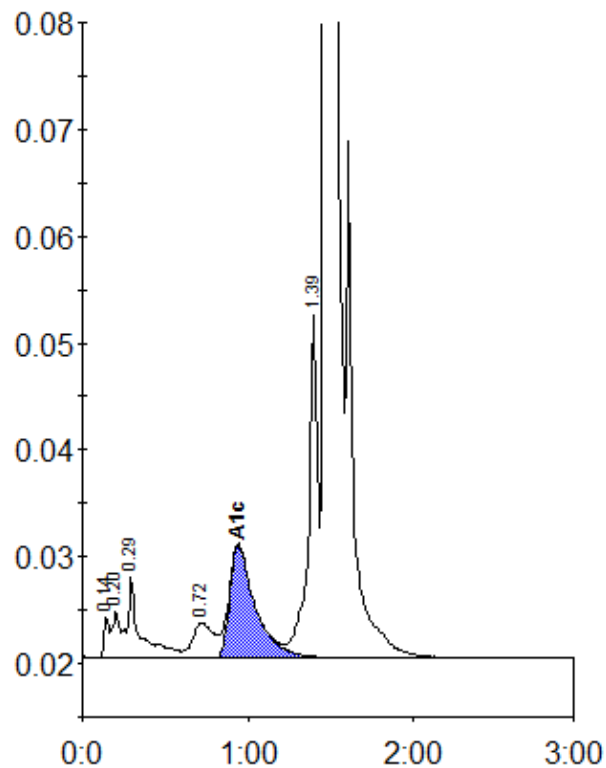
Peak table - ID: 10130406
