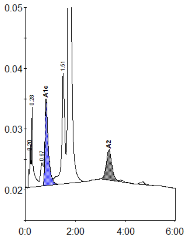
Peak table - ID: 10131667
