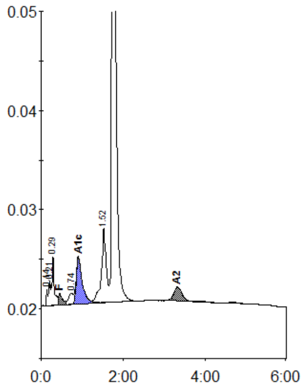
Peak table - ID: 10006171
